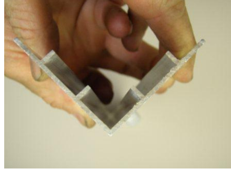
PTT - Trim Applicator lugs that push the render through the trim leg cut outs
